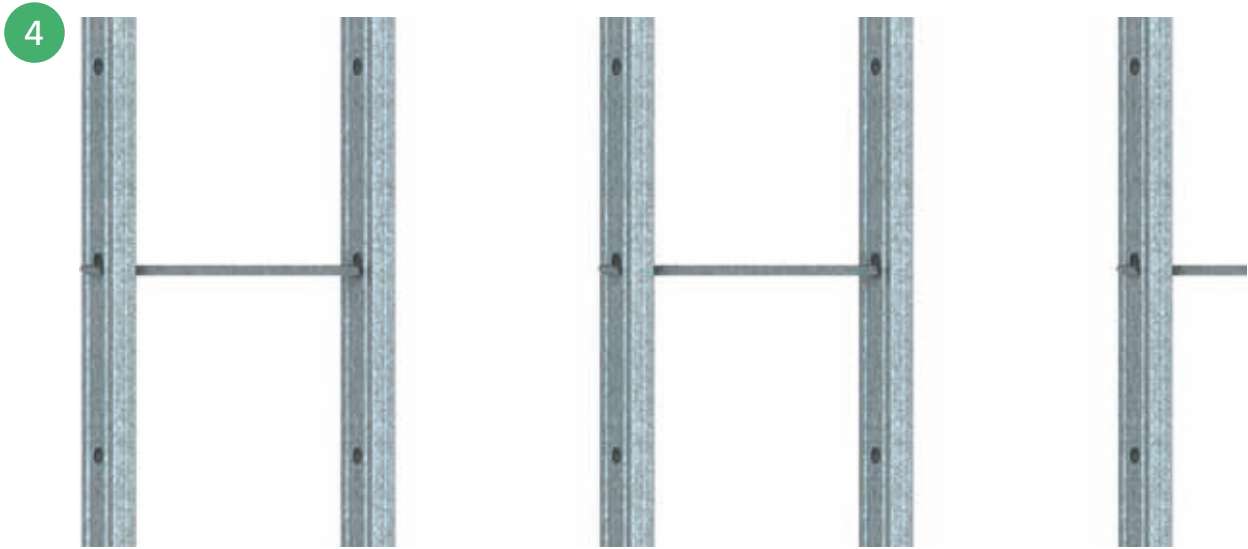
■ SINGLE SNAP-LOCK NOGGING JOINING RONDO STEEL STUDS IN PAIRS
