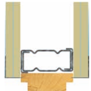
P28: DETAIL AT DOOR JAMB
