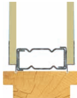
DETAIL AT DOOR JAMB
