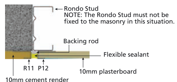
CONTROL JOINT: RENDER/PLASTERBOARD
