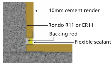
CONTROL JOINT CORNER DETAIL
